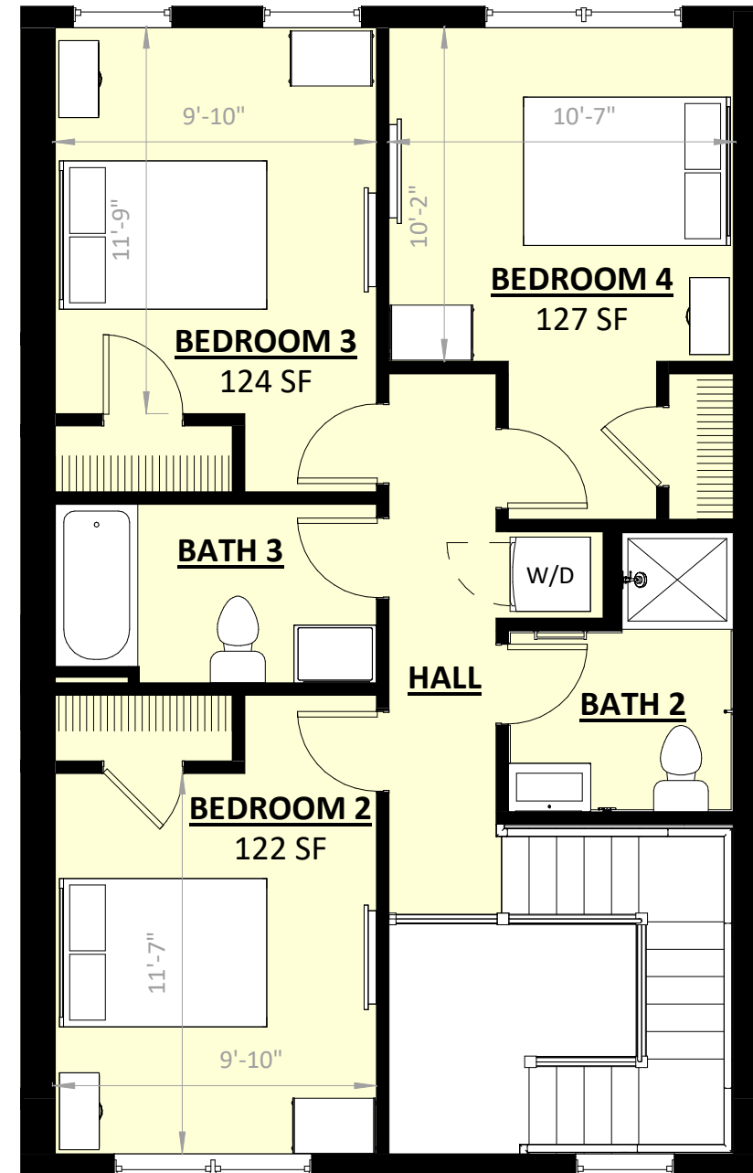
2 UNIT C - 2ND FLOOR 3/16" = 1'-0"
