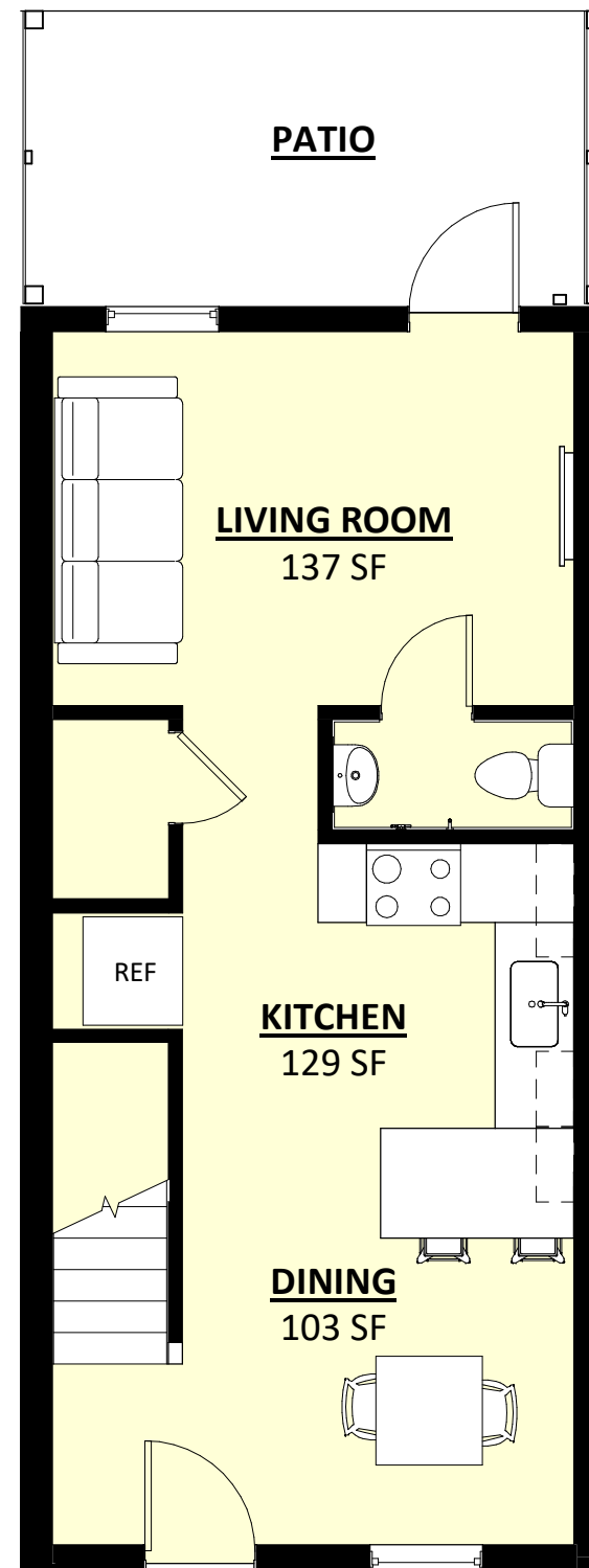
1 UNIT B - 1ST FLOOR 3/16" = 1'-0"
