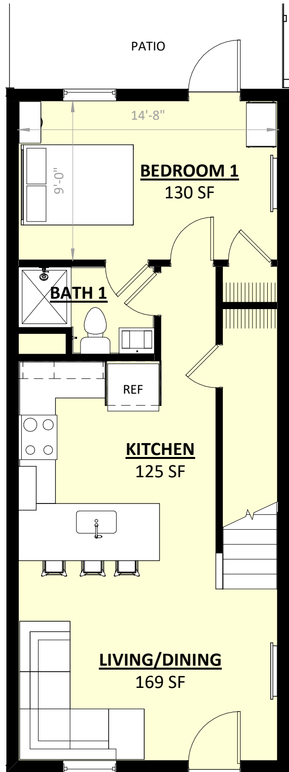
1 UNIT A - 1ST FLOOR 3/16" = 1'-0"
