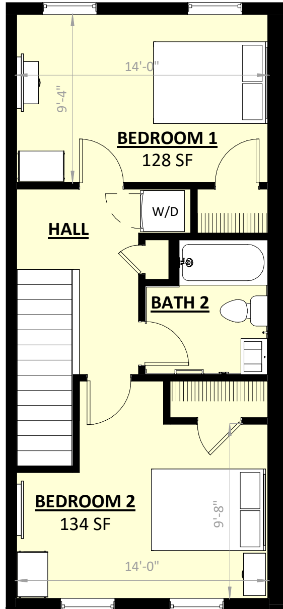
2 UNIT B - 2ND FLOOR 3/16" = 1'-0"
