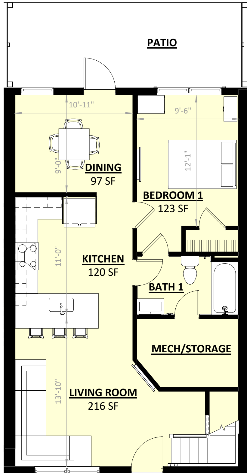
1 UNIT C - 1ST FLOOR 3/16" = 1'-0"
