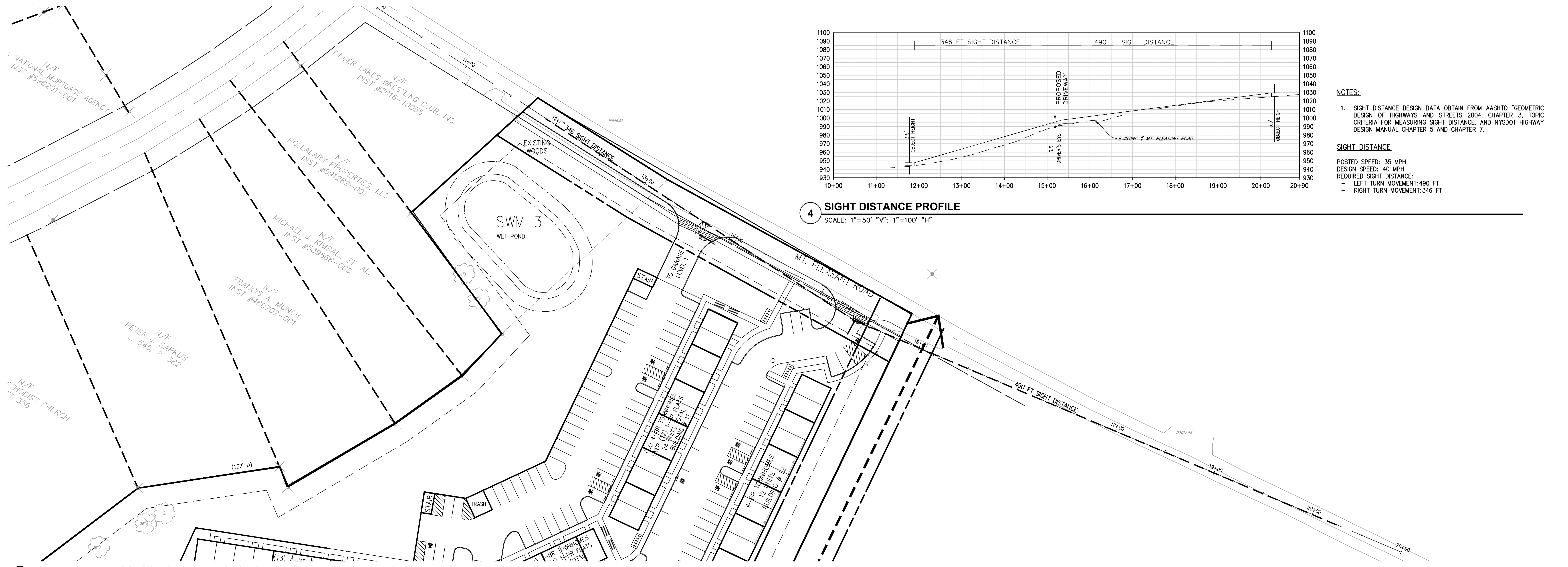
3 PLAN VIEW AT ACCESS ROAD INTERSECTION WITH MT. PLEASANT ROAD
