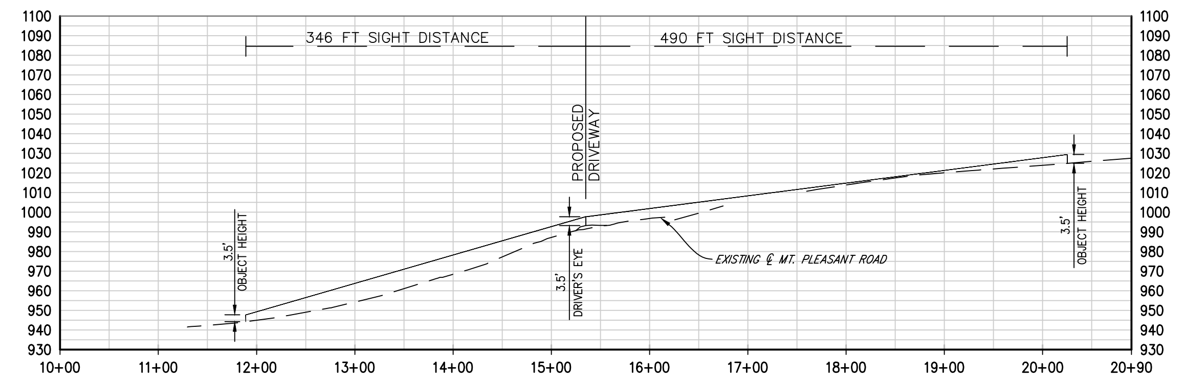
4 SIGHT DISTANCE PROFILE
