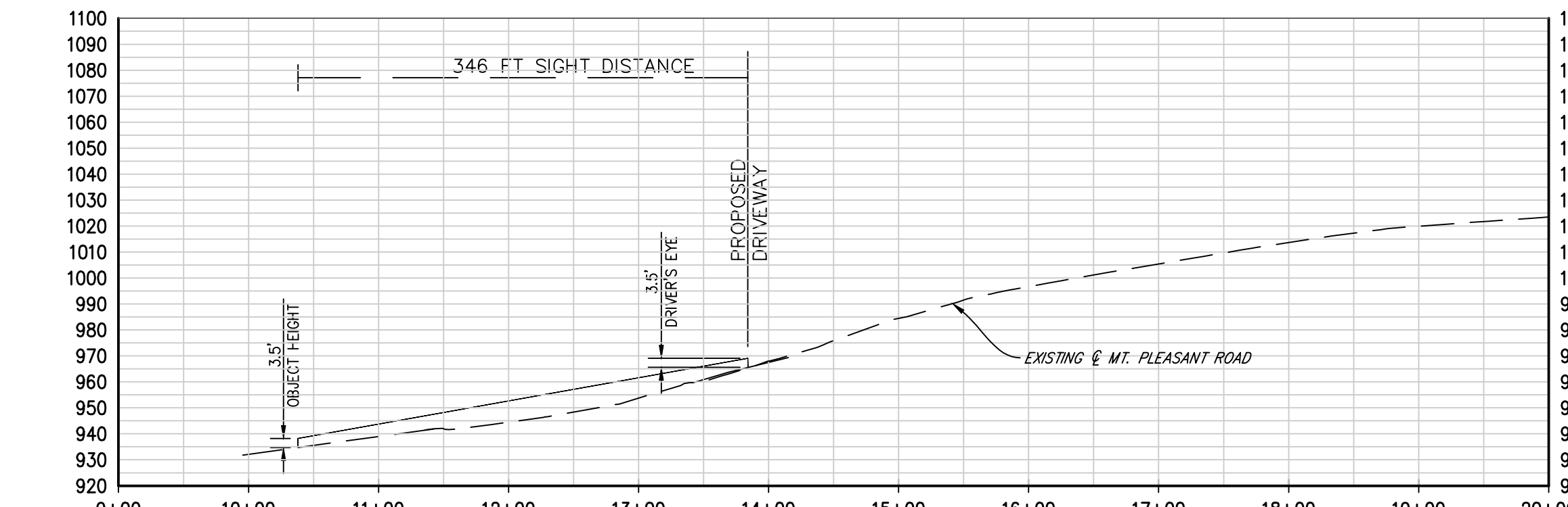
2 SIGHT DISTANCE PROFILE
