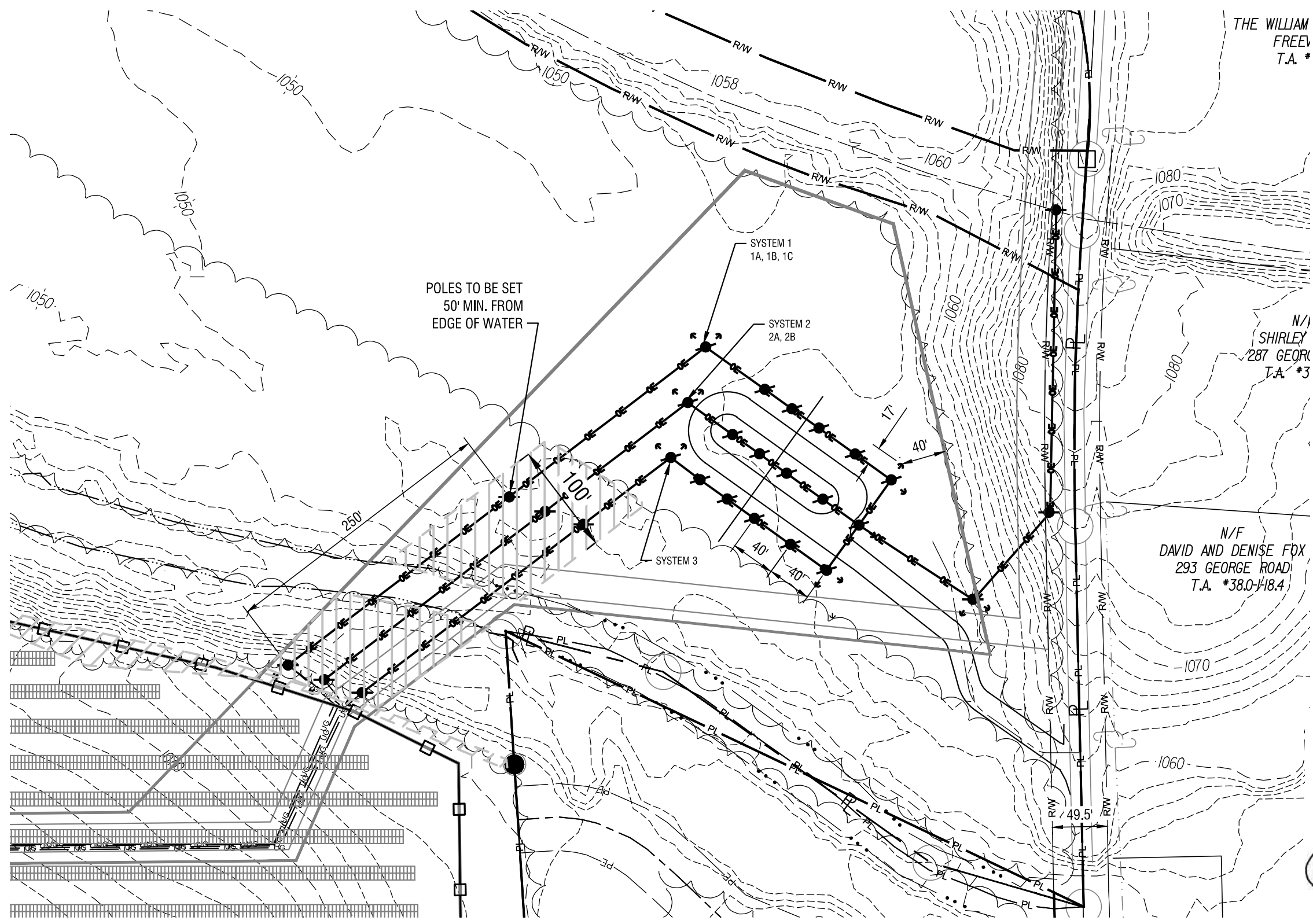
1 POLE FARM SITE PLAN SCALE: 1" = 100'
