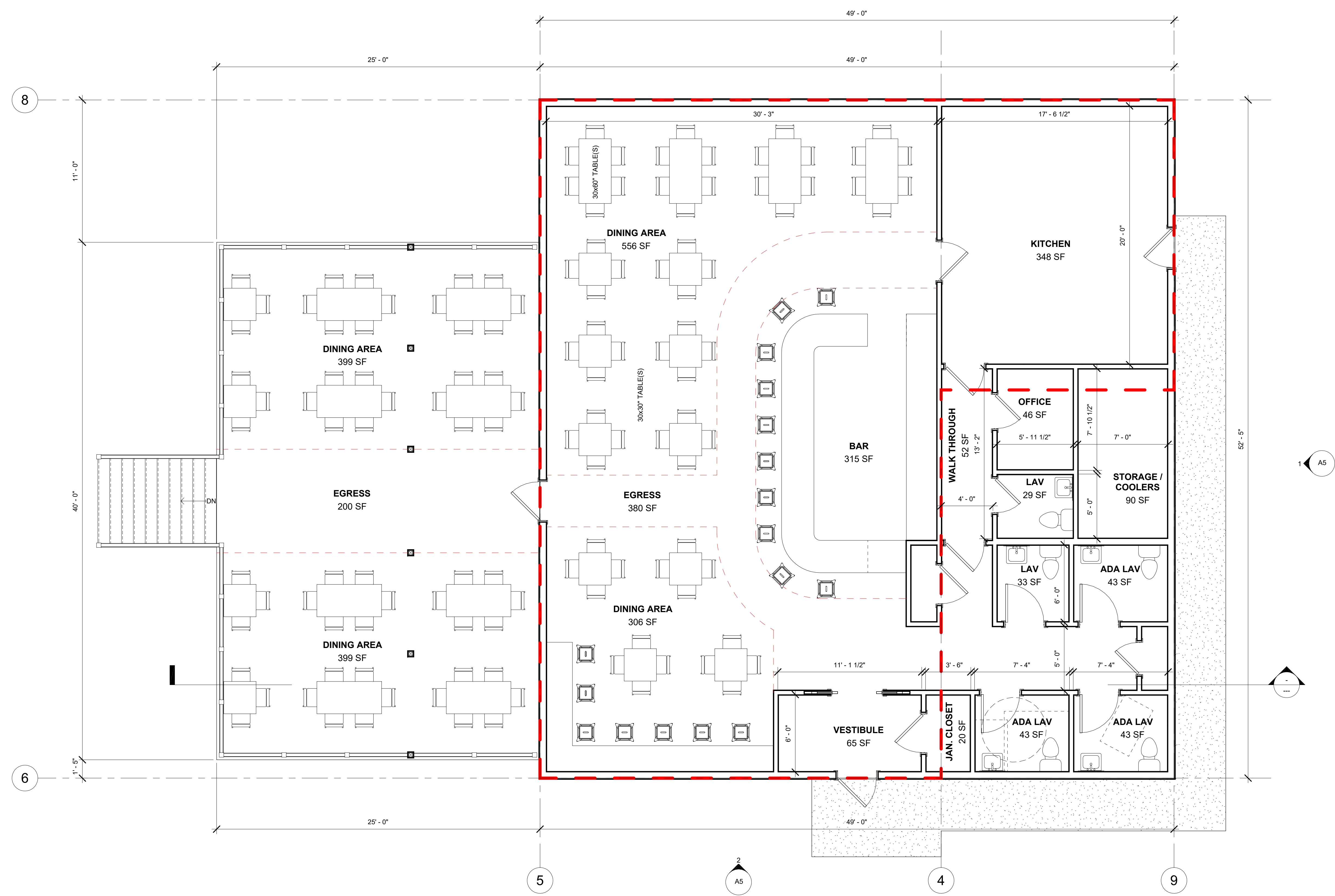
1 FLOOR PLAN - 1ST FLOOR 1/4" = 1'-0"
